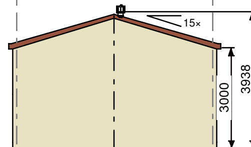
ELEVATION GRID 3
